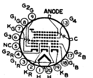
20A ANODE = G_3 + G_4 + CL FOCUSING ELECTRODE = G_3
