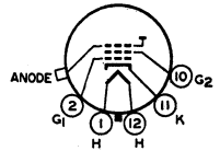
12D ANODE = G_3 + CL
