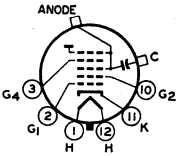
12AB ANODE = G_3 + G_2 + CL FOCUSING ELECTRODE = G_4
