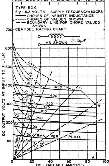
OPERATION CHARACTERISTICS FULL-WAVE CIRCUIT, CHOKE INPUT TO FILTER
