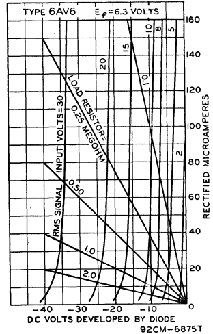
AVERAGE DIODE CHARACTERISTICS HALF-WAVE RECTIFICATION—SINGLE DIODE UNIT
