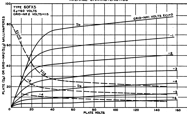
AVERAGE CHARACTERISTICS
