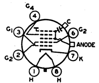
8JK ANODE = G_3 + G_2 + CL FOCUSING ELECTRODE = G_4
