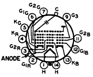
14AU ANODE = G_4 + G_2 + CL FOCUSING ELECTRODE = G_3
